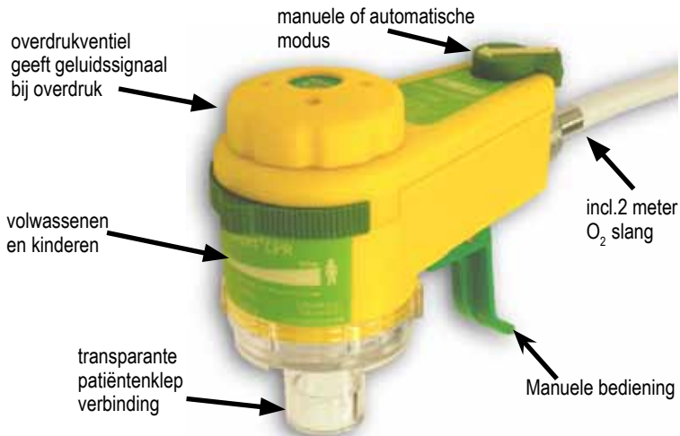
Model: microVENT CPR - 670-0483-00
